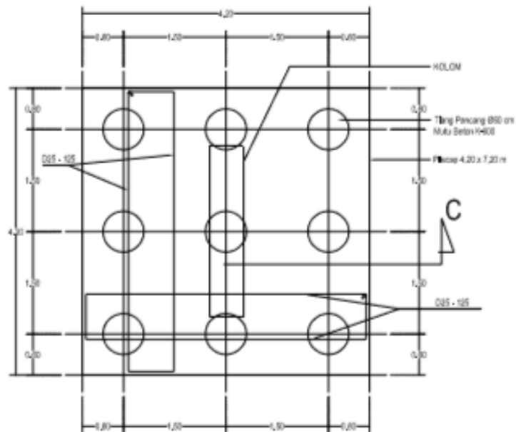
DETAIL PONDASI TYPE P2 Skala 1:50
